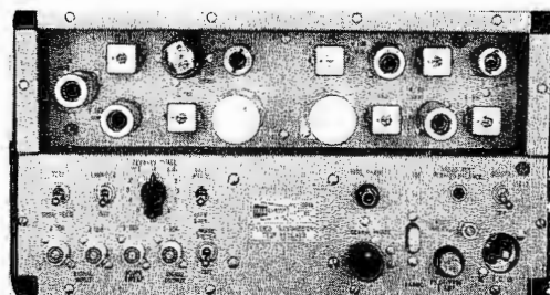
Telechrome Manufacturing Corp. — Model 1004-B Video Transmission Test Signal Receiver
