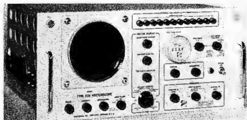
Tektronix — Type 526 Color-Television Vectorscope
