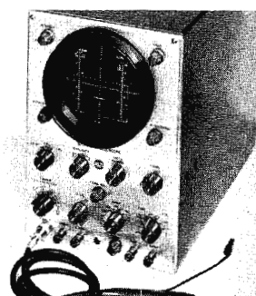
Shown, left to right, are a Western Reserve Electronics militarized tube tester, the Hewlett-Packard 204B Oscillator, a Conrac Video Monitor showing pulse-cross display, and an RCA WO-91A general purpose oscilloscope.
